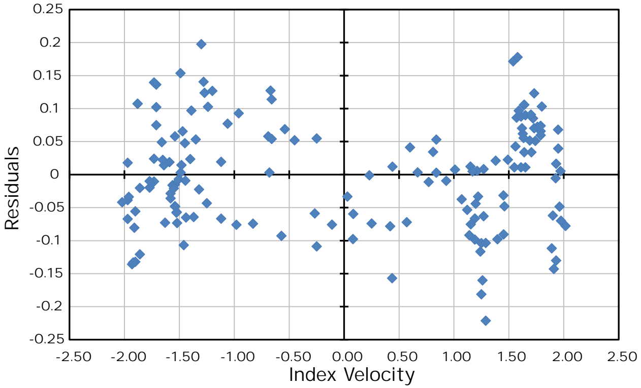
Residual Plot
